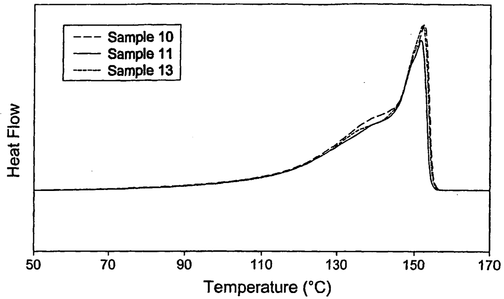
Fig. 7 DSC Melting of Plasticized Propylene Random Copolymers
